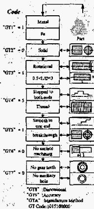
Figure 4 Coding process for a rotational part
