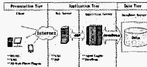
Figure 1 Architecture of manufacturing e-Learning system (eCAM)
