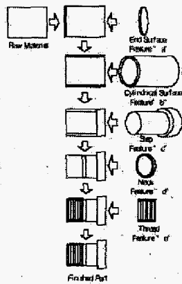
Figure 2 Manufacturing features of turning process
